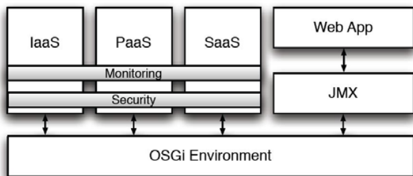
Fig. 1 CAPI Architecture
