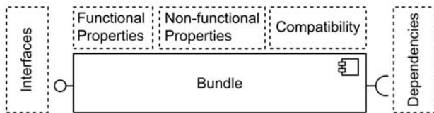
Fig. 4 OSGi Bundle Description
