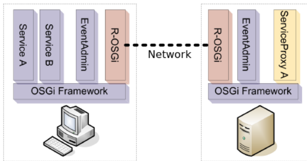
Fig. 6 Example for usage of R-OSGi [10]
