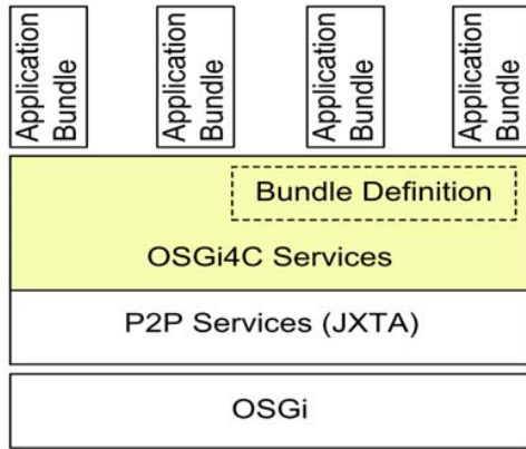
Fig. 3 OSGi4C Architecture
