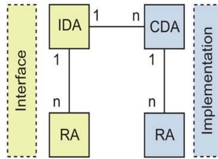
Fig. 5 JXTA advertisements
