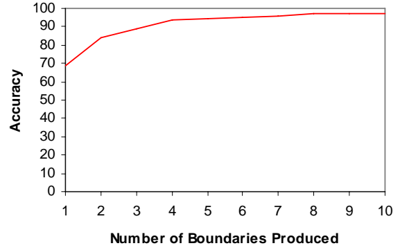
Fig. 3 The percentage of the 120 images, in which at least one out of the K detected contours catches 20% of the target boundary. The curve is obtained by varying K from 1 to 10 continuously.
