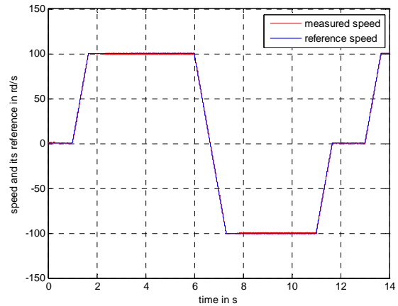
Fig. 5: speed and its reference
