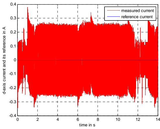
Fig. 6: d-axis current and its reference
