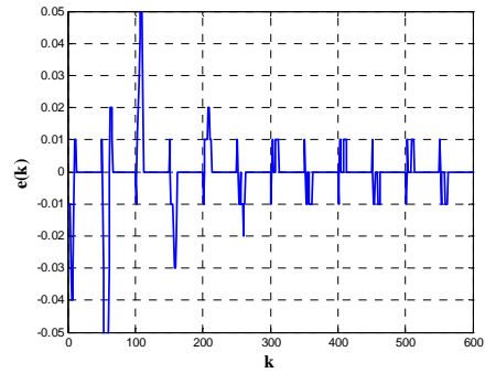
Fig. 49 Error between Model & System for g_2 = 7 .
