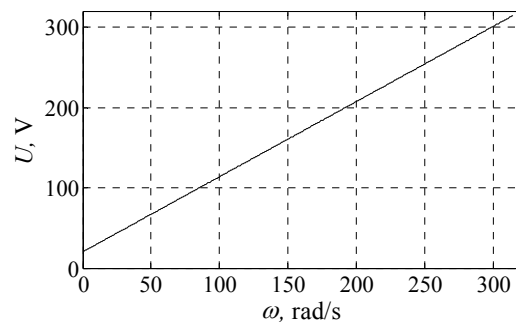
Fig. 5 Dependence voltage against frequency
