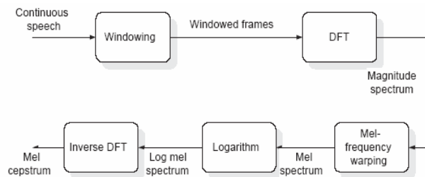
Fig. 7 MFCC calculation
