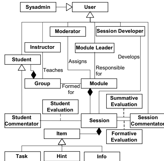
Figure 1: UML Class Diagram
