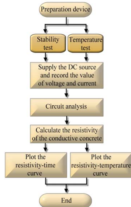
Fig. 3. Flowchart of the resistivity measurement.
