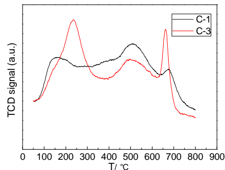
Fig. 5 H 2 -TPD profiles on Fe/SiO 2 and FeNi/SiO 2 catalysts reduced in H 2
