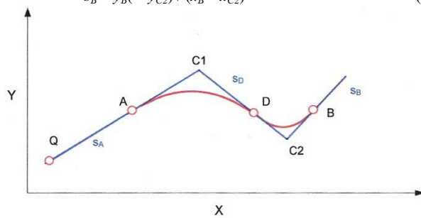
Fig. 3 Wireframe representation of reverse vertical curve
