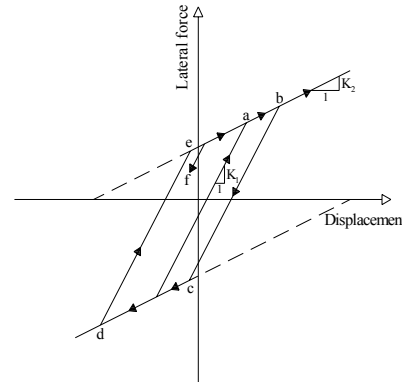
Fig. 2 Nonlinear bilinear Elasto-Plastic stiffness model
