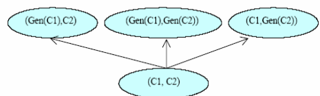
Fig. 6 Each tuple will be divided into tree tuples. "Gen" stands for General
