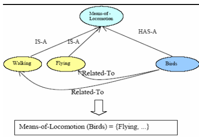
Fig. 11 Example for Pattern 1
