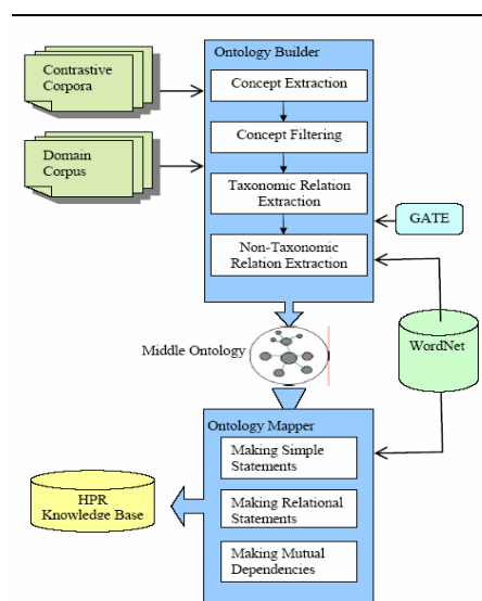
Fig. 1 General schema of our system's architecture
