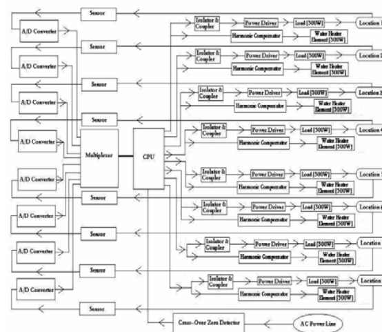
Fig. 1 Block diagram of the dimmer
