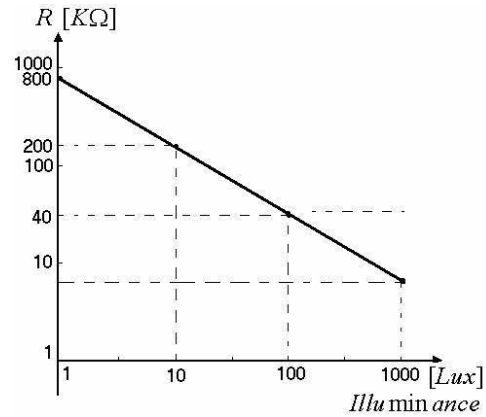
Fig. 4 Cds 8107 resistance vs. illuminance characteristic
