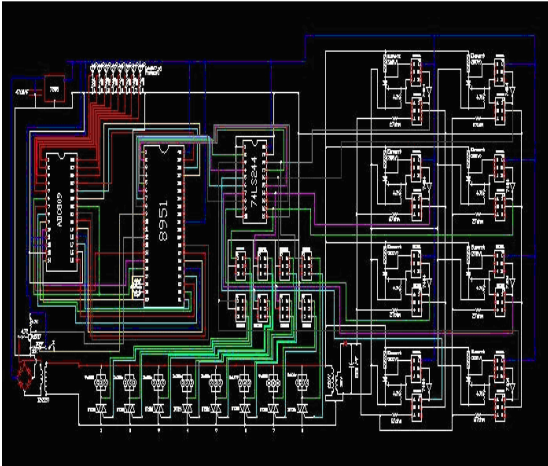
Fig. 2 Hardware of the dimmer
