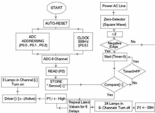
Fig. 3 Flow chart for software of the dimmer
