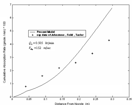
Fig. 2 Cumulative absorption of SO_2 along the venturi scrubber
