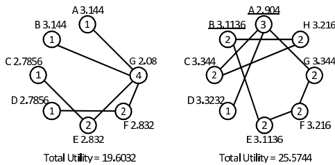
Fig. 4. Stable network shape of 1111224 and 12222223
