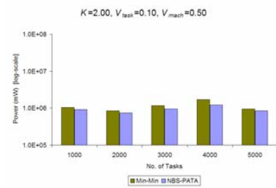
Fig. 7 Power consumption
