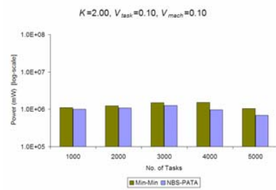
Fig. 6 Power consumption
