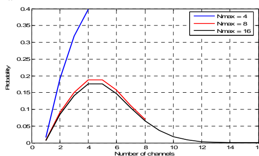
Fig. 3 Distribution of active channels when A = 5 \text{ Erl} and N_{max} = 4, 8, 16
