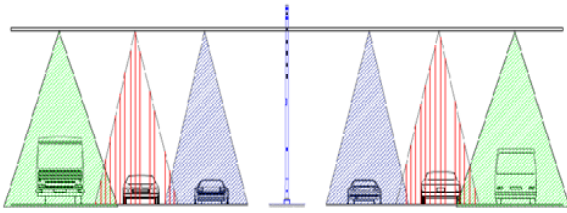
Fig. 4 Lane detection
