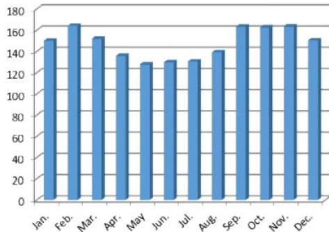
Fig. 2 Radiation – Vertically Surface – Tehran – MJ/m^2
