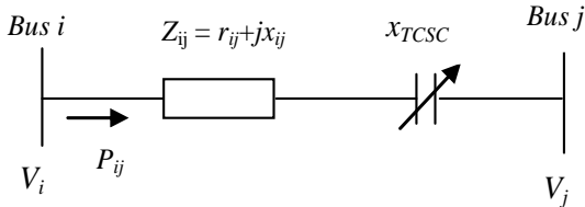
Fig. 1 Model of transmission line with TCSC
