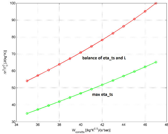
Fig. 36 Ratio of L to inlet total temperature vs. corrected mass flow rate – maximum efficiency, and balanced individual
