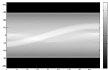
Fig. 6 Sinogram of the specimen with defects
