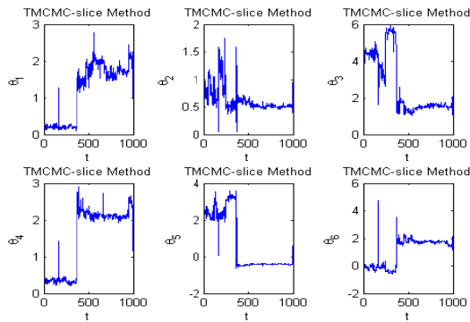
Fig. 5 Sample path of the damage identification results based on TMCMC-slice
