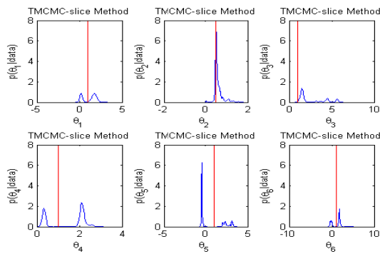
Fig. 6 Probability density of the damage identification results based on TMCMC-slice
