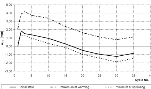
Fig. 11 Deflection at central point 3 along z-axis
