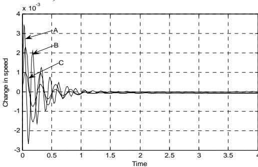
Fig. 9 Dynamic response for \Delta\omega
