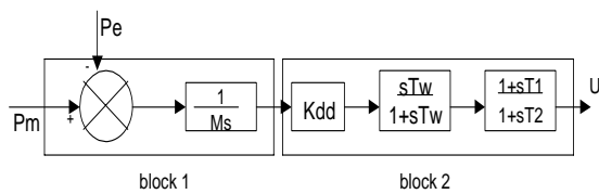
Fig. 3 Transfer function block diagram of the POD
