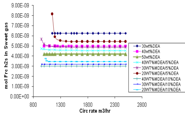
Fig. 12 The effect of different percent of mixing amines and different percent of DEA upon the amount of H 2 S in the sweet gas in different circulation rate
