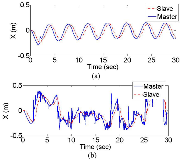
Fig. 8 the variable time delay ranges from 0 to 0.3 sec
