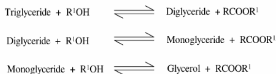
Fig. 2 General equation for transesterification of triglycerides
