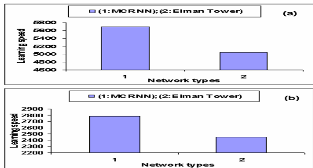
Fig. 5 (a) represents the learning speed when both networks run simultaneously on data set (A). (b) represents the learning speed when both networks run simultaneously on data set (B)
