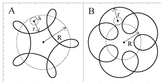
Fig. 5 (A) An hypotrochoid and; (B) an epitrochoid From [40]
