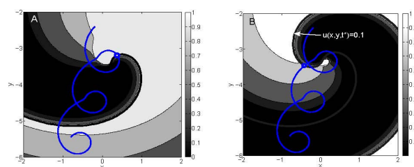
Fig. 6 Propagation of a spiral wave generated with Eqns. (2) with \tau_d = 0.3965 . The line in blue represents the trajectory of the tip. The different colored regions represent different levels of refractoriness given by the v variable. For v close to 0 (black), the region is in its maximum level of refractoriness and an AP cannot be elicited here. For v \approx 1 (white), the region is almost or totally recovered and an AP can be elicited in this region. (A) Formation of a petal; (B) Formation of an arc. The blue dot filled in white, is the location of the tip of the spiral
