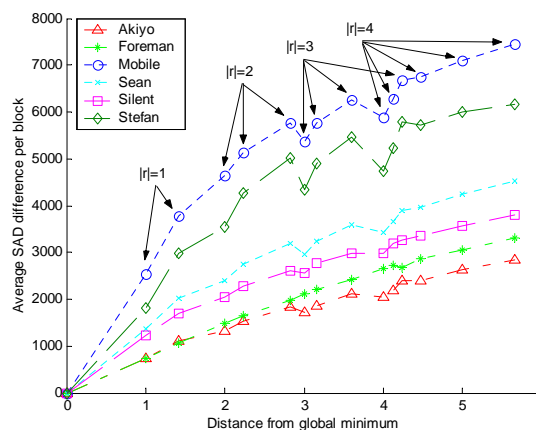
Fig. 2 Analysis of the relation between block SAD and distance
