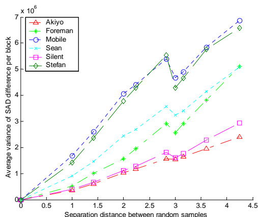
Fig. 3 Variance of block SAD difference for the random sample pairs taken from the 4x4 region around the global minimum
