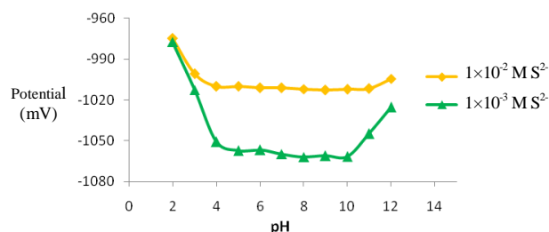
Fig. 3 Effect of pH to the response of sensor [Ca(2,2'-bipyridine) 3 ] 2+ -montmorillonite in 1 \times 10^{-2} M and 1 \times 10^{-3} M of \text{S}^{2-} solution
