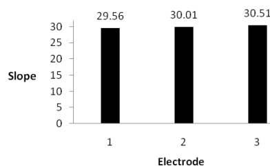
Fig. 4 Average slopes of 3 electrodes at pH 4
