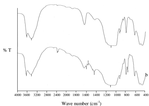
Fig. 2 FT IR spectra of Ca(II)-montmorillonite (a) and [\text{Ca}(2,2'\text{-bipyridine})_3]^{2+} -intercalated montmorillonite (b)
