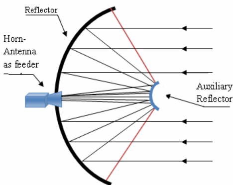
Fig. 3 The cassegrain feeding parabolic
