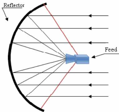
Fig. 2 Conventional Parabolic
