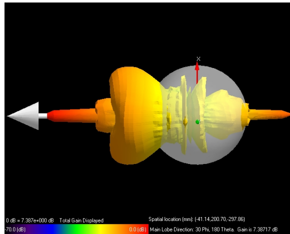
Fig. 9 The 3-D radiation pattern of the (CLLA) in xz-axis display
