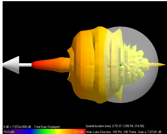
Fig. 8 The 3-D radiation pattern of the (LLA) in xz-axis display
