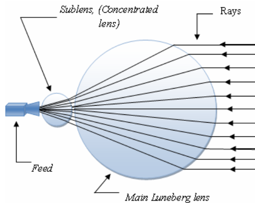
Fig. 5 Luneberg lens with Concentrating lens antenna
