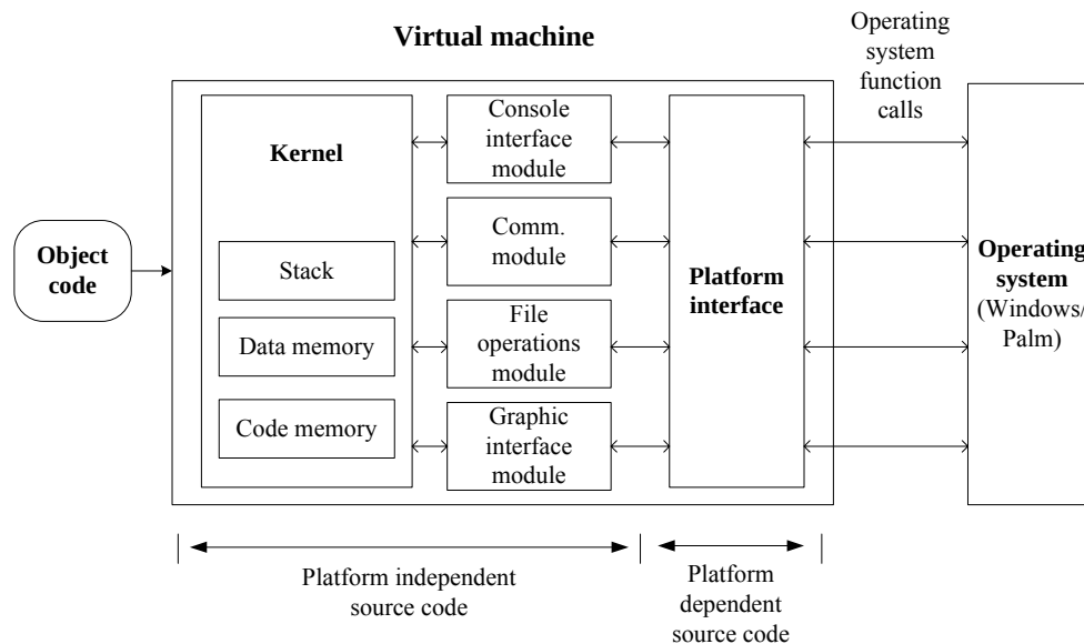
Fig. 4 The architecture of the virtual machine
