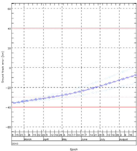
Fig. 8 Target Frozen Eccentricity \Delta a = -40 m
