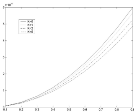
Fig. 4. Critical Buckling Load of FG Beam with Piezoelectric Actuators Versus h/L for V = 10 v .
