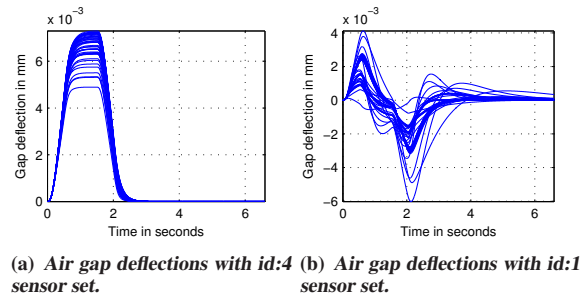
Fig. 7. Air gap deflection with single measurements.
