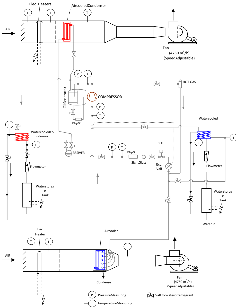
Fig. 1 Experimental system
