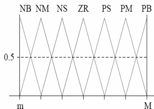
Fig. 3 Graphical representation of a uniform fuzzy partition
