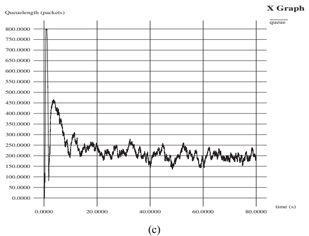
Fig. 8 Instantaneous queue size, PSO/first-order controller, (a) PSO/first-order controllers (b) First-order controllers (c) PI controllers
