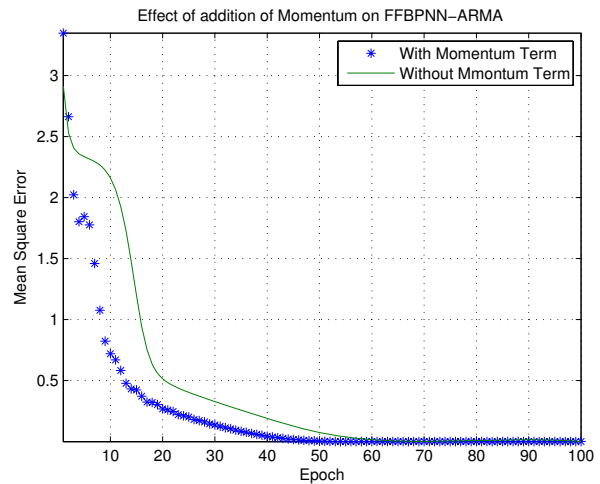
Fig. 7. Effect of addition of Momentum term
