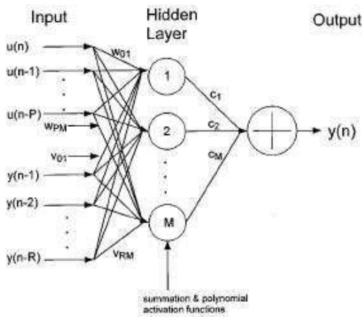
Fig. 2. Neural Network Technique for obtaining ARMA/NARMA coefficients. [6], [7]
