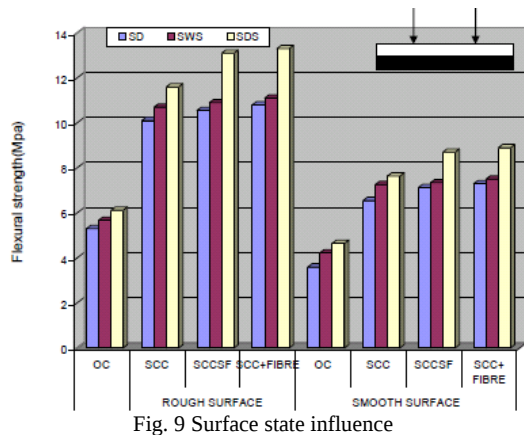
Fig. 9 Surface state influence
