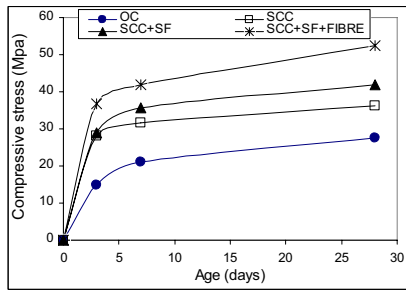
Fig. 1 Compressive stress
