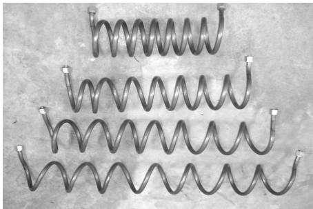
Fig. 2 Pitches of the coiled tube
