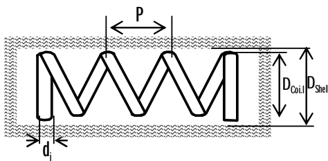
Fig. 3 Coiled tube heat exchanger
