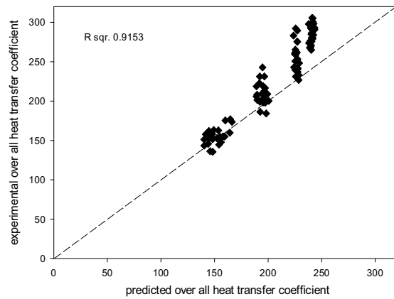
Fig. 5 Comparison of experimental data with present data of 6.31 cm pitches coil
