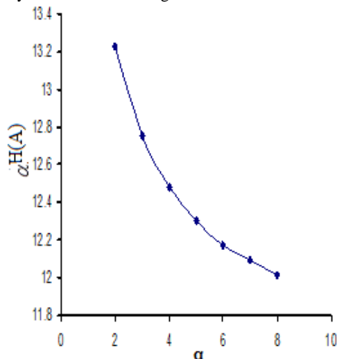
Fig.4 Graph {}_a H(A) Versus \alpha
