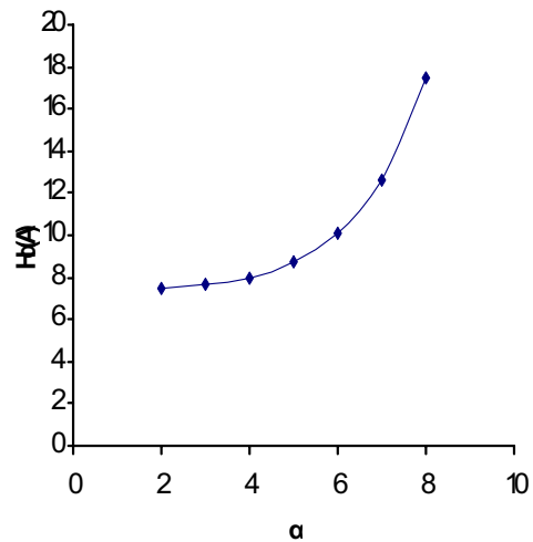
Fig.3 Graph H_\alpha(A) Versus \alpha
