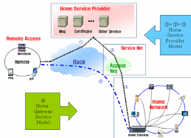
Fig. 5 Home-Network Model
