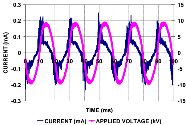
(a) Current & voltage waveforms
