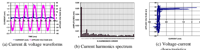
Fig. 2. Typical waveform of low RH clean specimen
