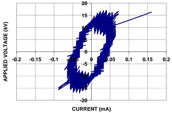
Fig. 10. Typical waveform of low RH heavily polluted specimen
