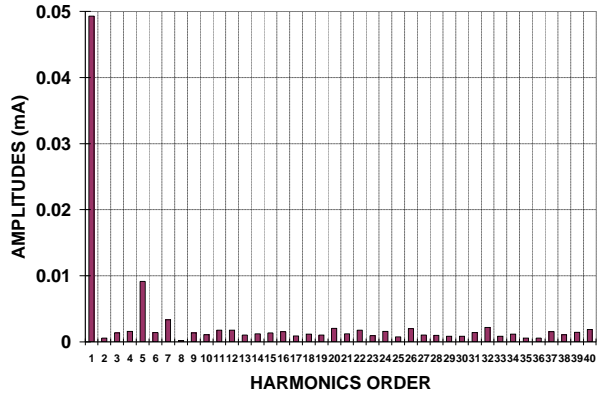
(b) Current harmonics spectrum
