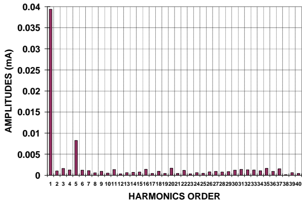
(b) Current harmonics spectrum
