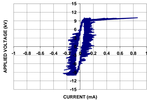
(c) Voltage-current characteristics
