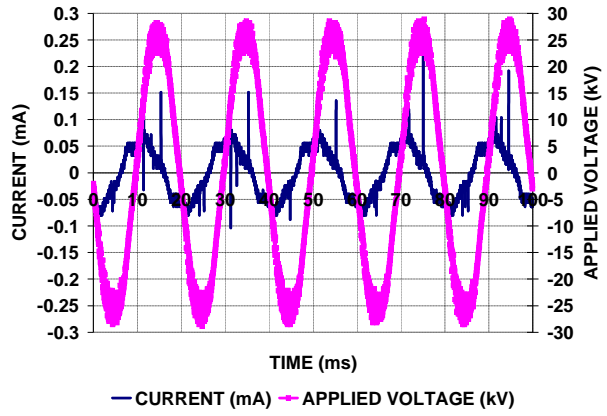
(a) Current & voltage waveforms
