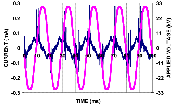
(a) Current & voltage waveforms
