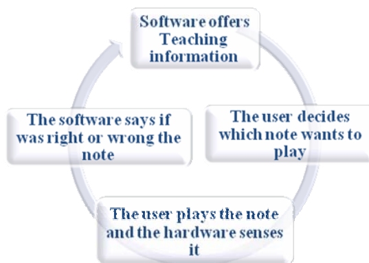
Fig. 4 System Dynamic
