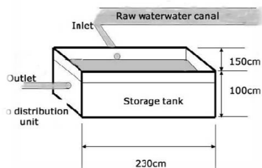
Fig. 2 Storage/ sedimentation unit
