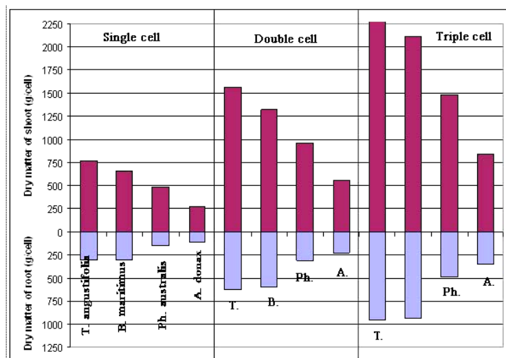
Fig. 8 Weight of macrophyte tissues (root and shoot) harvested from constructed wetland experiment.
