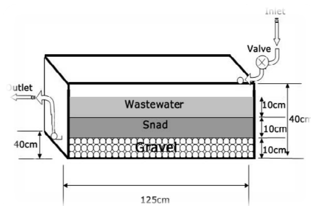
Fig. 5 Microcosm of constructed wetlands/ cells
