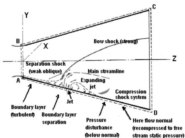
Fig. 1 Complex flow structure associated with SITVC
