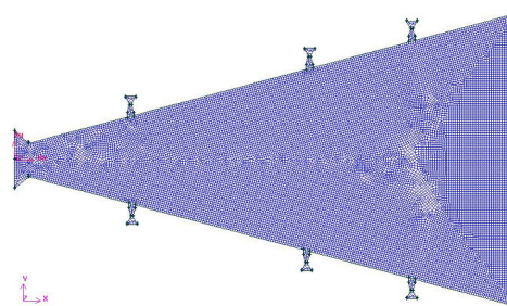
Fig. 3 Grid system in the computational domain
