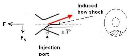
Fig. 4 Demonstrating the formation induced bow shock
