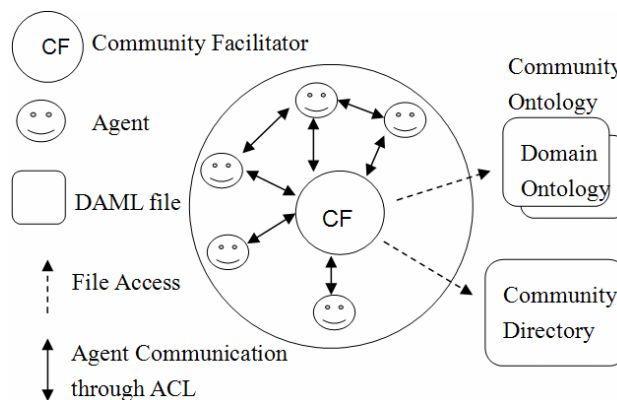
Fig. 2 Communication in Agent Community
